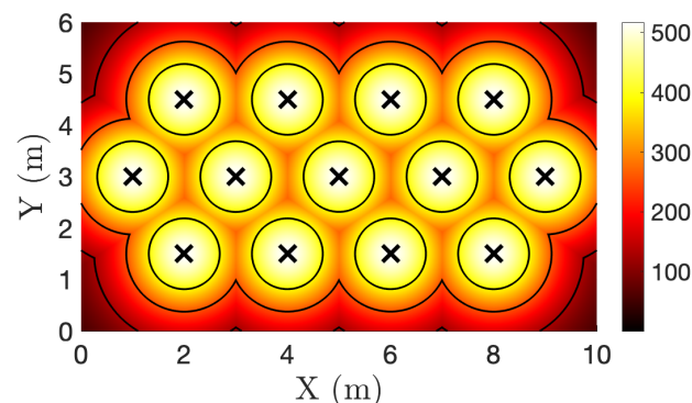
Figure 6. The illumination level distribution (in lx) in a 10 \text{ m} \times 6 \text{ m} room with 13 LED luminaires.
