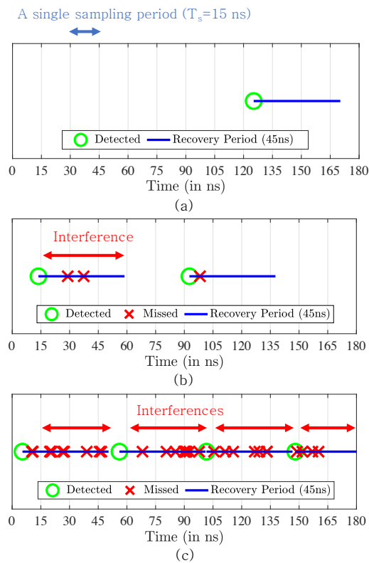
Figure 9. The simulation trials of the photon detection process with the influence of the SPAD’s dead time (45 ns) considering a single microcell within a SiPM 30035 chip when the received irradiance levels are (a) 1 mW/m 2 , (b) 10 mW/m 2 , and (c) 100 mW/m 2 . In these figures, the green circles indicate the time of detected photons and the blue lines indicate the associated dead time. The red crosses indicate the missed photons.
