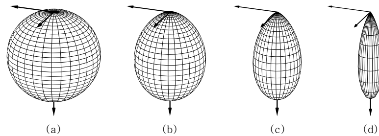
Figure 5. The radiation pattern of LEDs with different Lambertian orders (a) m = 1 ( \Phi_{1/2} = 60^\circ ), (b) m = 2 ( \Phi_{1/2} = 45^\circ ), (c) m = 5 ( \Phi_{1/2} = 30^\circ ), and (d) m = 20 ( \Phi_{1/2} = 15^\circ ).
