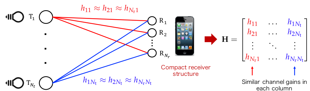
Figure 12. Optical channel between multiple LED transmitters and multiple photodetectors.
