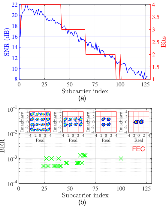
Fig. 6. (a) The estimated SNR and the loaded number of bits on different OFDM subcarriers when the transmission data rate is 25.6 Mbps using the YS-2 fiber antenna, (b) the BER of different OFDM subcarriers and the received signal constellations after channel equalization.
