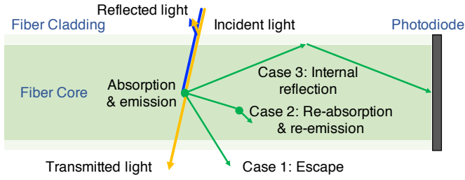
Fig. 1. The physical processes of the light within the fluorescent fiber.
