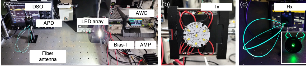
Fig. 3. (a) A photo of the VLC experiment setup, (b) a photo of the LED array on an aluminum PCB board, (c) a photo of the fluorescent fiber antenna under 400 nm blue light.
