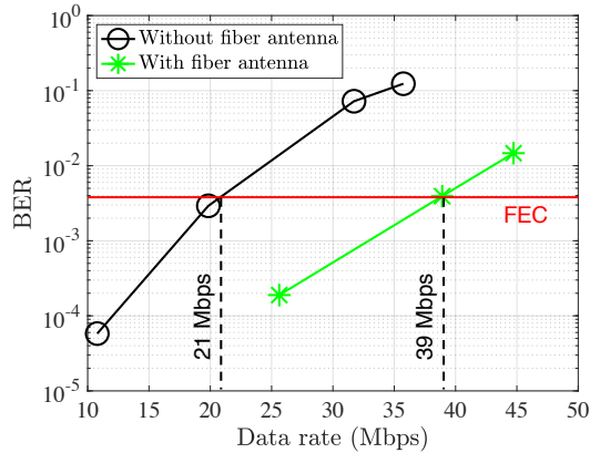
Fig. 7. The measured BERs at different transmission data rates with and without the fluorescent fiber antenna.
