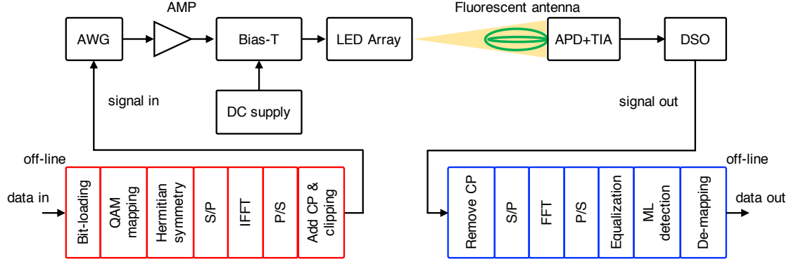
Fig. 4. The block diagram of the VLC experiment setup and the main off-line signal processing steps.
