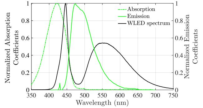
Fig. 2. The absorption and emission spectrum of the YS-2 fluorescent fiber and the spectrum of the white LED. The absorption and emission spectra of the YS-2 fiber were obtained from its datasheet and the spectrum of the LED was measured using a photonic multichannel spectral analyzer (Hamamatsu, PMA-11 model C7374-36).
