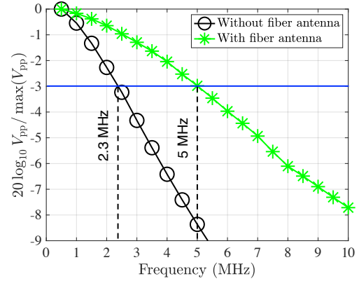
Fig. 5. The measured frequency response with and without the YS-2 fluorescent fiber antenna.
