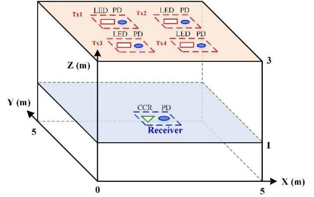
Fig. 3. Simulation setup.
