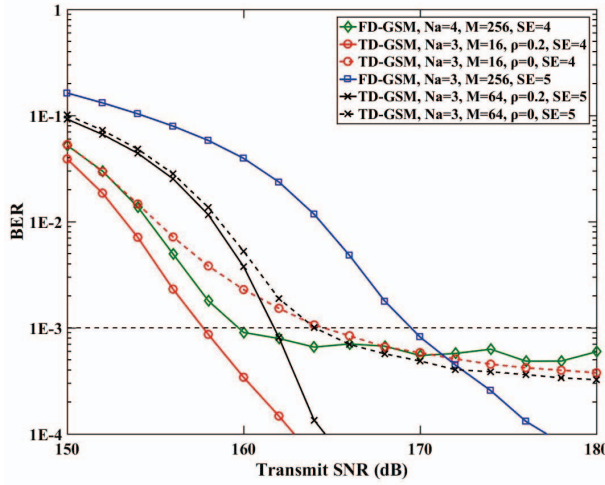
Fig. 5. BER performance comparison between OFDM-based FD-GSM and TD-GSM for different spectral efficiencies (bits/s/Hz).
