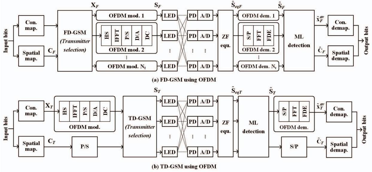
Fig. 1. Schematic diagrams of (a) OFDM-based FD-GSM and (b) OFDM-based TD-GSM.
