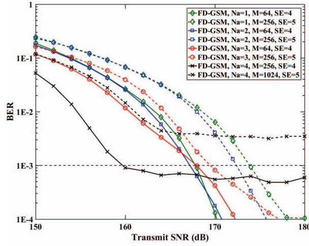
Fig. 3. BER vs. transmit SNR for OFDM-based FD-GSM for different spectral efficiencies (bits/s/Hz).
