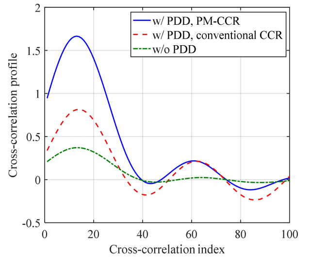
Fig. 9. Cross-correlation curves of two CCRs at a distance of 78 cm with and without PDD.
