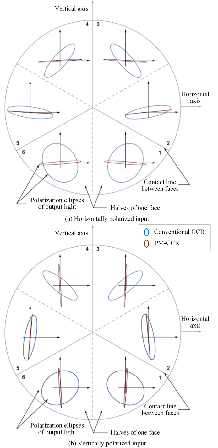
Fig. 2. Output polarization ellipse distributions of conventional CCR and PM-CCR under (a) horizontally polarized input and (b) vertically polarized input.
