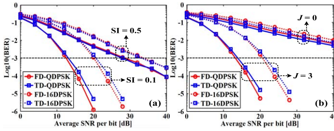
Fig. 4. BER performance of NE-OFDM using FD-MDPSK and TD-MDPSK: (a) J=4 with different SI values and (b) SI=0.1 with different J values.
