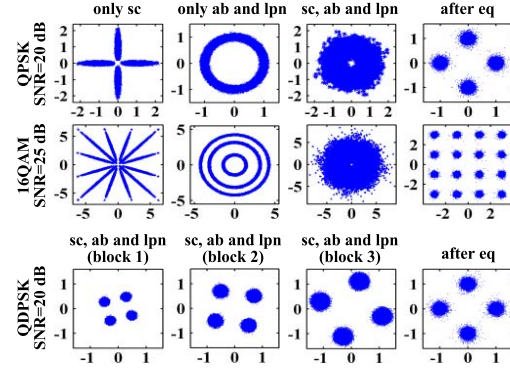
Fig. 6. Constellation diagrams of QPSK/16QAM based OFDM and QDPSK based NE-OFDM for SI=0.1 and J=6 (sc: scintillation; ab: aberration; lpn: laser phase noise).
