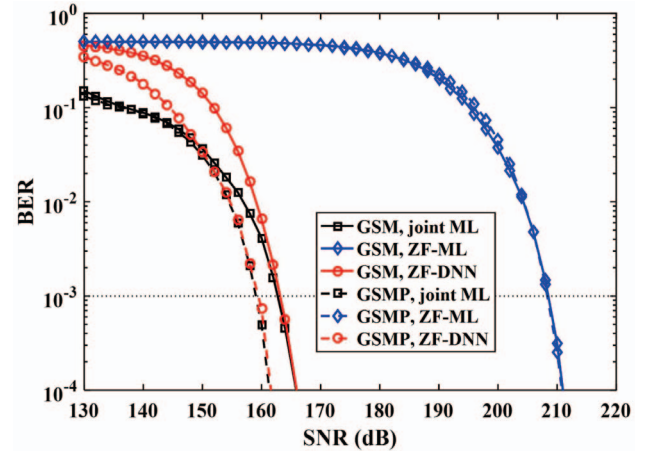
Fig. 6. BER vs. transmit SNR for GSM and GSMP in the 4 \times 4 MIMO-VLC system with different detection schemes. The receiver position is (0 m, 0 m, 0.7m) and the spectral efficiency is 4 bits/s/Hz.
