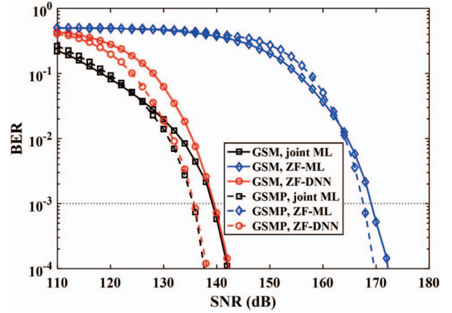
Fig. 5. BER vs. transmit SNR for GSM and GSMP in the 4 \times 4 MIMO-VLC system with different detection schemes. The receiver position is (2 m, 2 m, 0.7 m) and the spectral efficiency is 4 bits/s/Hz.
