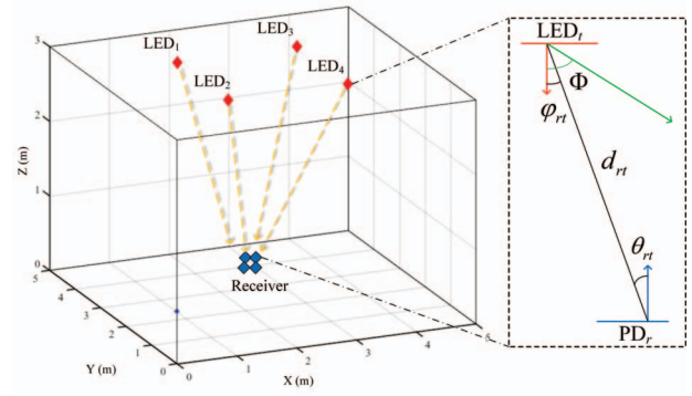
Fig. 3. Geometric setup of the 4 \times 4 MIMO-VLC system.
