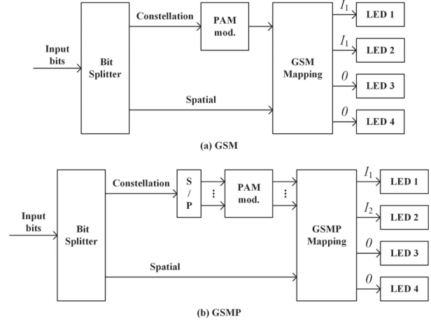
Fig. 1. Schematic diagram of (a) GSM and (b) GSMP using M -PAM modulation with N_t = 4 and N_a = 2 .
