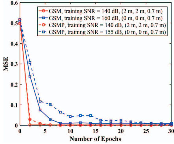
Fig. 4. MES loss of the ZF-DNN detector for GSM and GSMP with two receiver locations.
