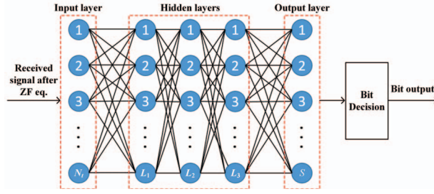
Fig. 2. Block diagram of the ZF-DNN detector for generalized optical MIMO.
