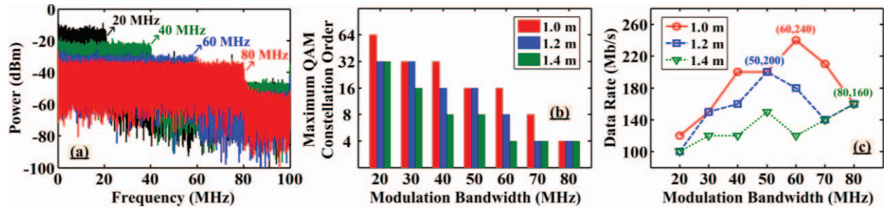
Fig. 2. (a) Electrical spectra after performing pre-FDE, (b) maximum QAM constellation order versus modulation bandwidth and (c) achievable data rate versus modulation bandwidth.
