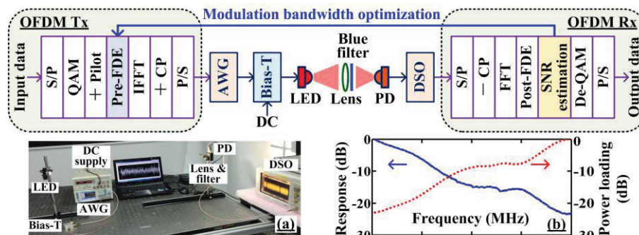
Fig. 1. Experimental setup. Insets: (a) photo of the overall system and (b) frequency response and power loading coefficients of pre-FDE.
