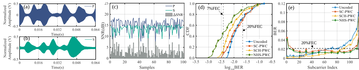
Fig. 2. (a) Normalized received waveform of different polarization direction denoted as parallel (P) and (b) senkrecht (S), (c) SNR results of collected samples, (d) CDF of measured BER results from collected samples and (e) BERs versus data SCs employing different schemes
