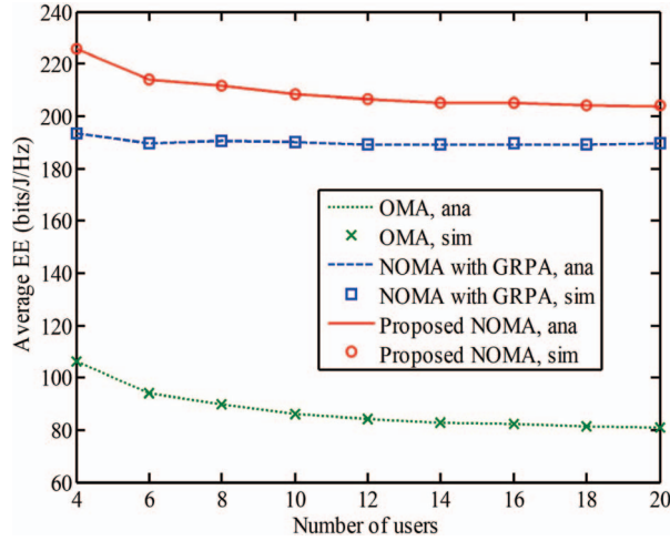
Fig. 4. Average EE vs. number of users with QoS set \tilde{R} = 1 .
