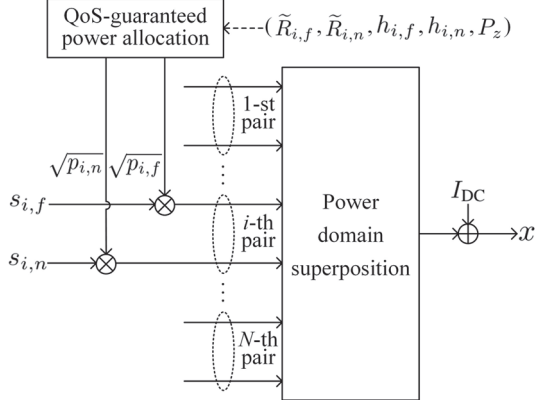
Fig. 2. Schematic of energy-efficient NOMA-enabled multi-user VLC.
