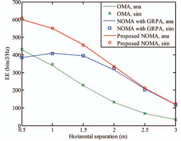
Fig. 3. EE vs. horizontal separation of two users with \tilde{R}_f = \tilde{R}_n = 1 bit/s/Hz.
