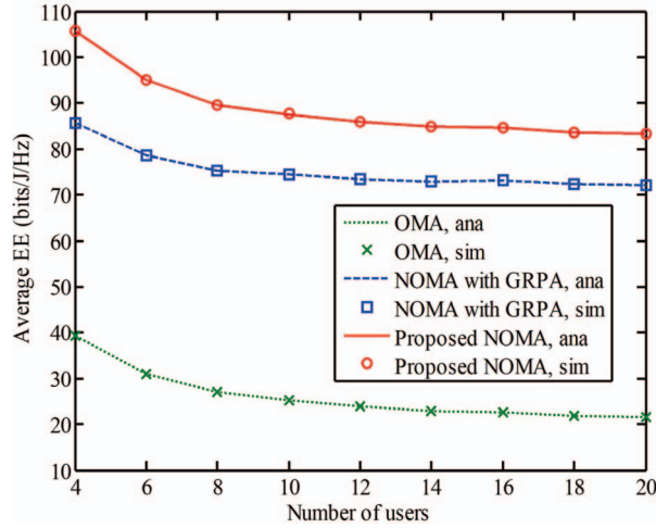
Fig. 5. Average EE vs. number of users with QoS set \tilde{R} = \{1, 2\} .
