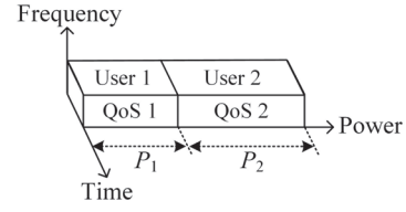
Fig. 1. Conceptual diagram of power domain energy-efficient NOMA.
