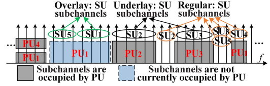
Fig. 2. The hybrid overlay/underlay spectrum access mode.
