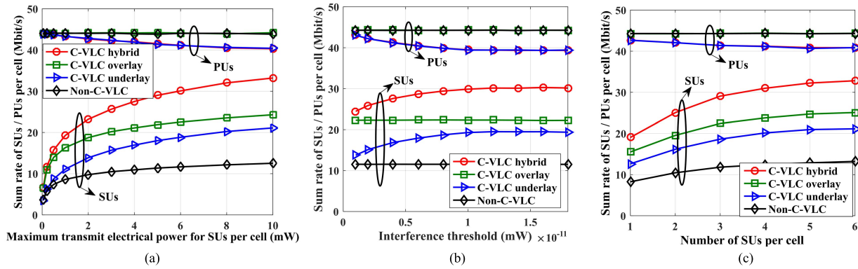
Fig. 3. Sum rate of SUs and PUs versus: (a) maximum transmit electrical power for SUs per cell, (b) interference threshold, and (c) number of SUs per cell.
