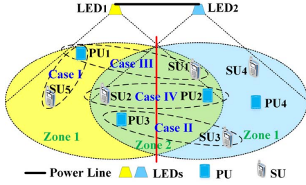
Fig. 1. A two-cell C-VLC system with hybrid overlay/underlay mode.
