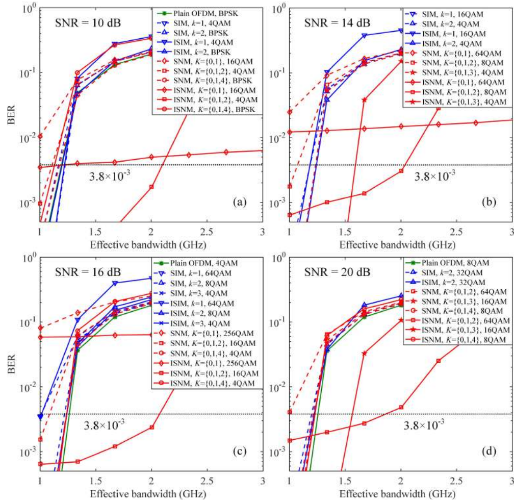
Fig. 5. Simulation BER vs. effective bandwidth for different schemes with a spectral efficiency of (a) 1 bit/s/Hz, (b) 1.5 bits/s/Hz, (c) 2 bits/s/Hz, and (d) 3 bits/s/Hz.
